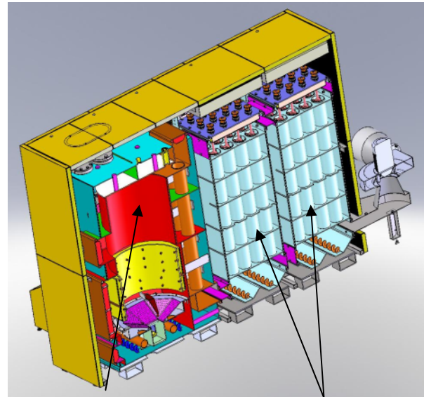
burner unit
